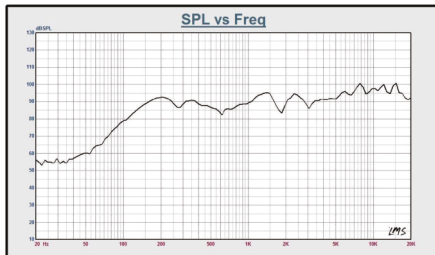
АЧХ (1Вт/ 1м) / RESPONSE CURVE (1w/1m)
